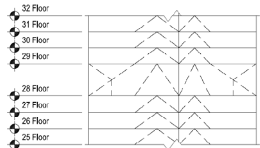
Figure 10: Typical E/W Outrigger Section (28th Floor)
