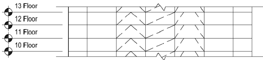
Figure 6: Typical Core N/S Core Bracing Elevation
