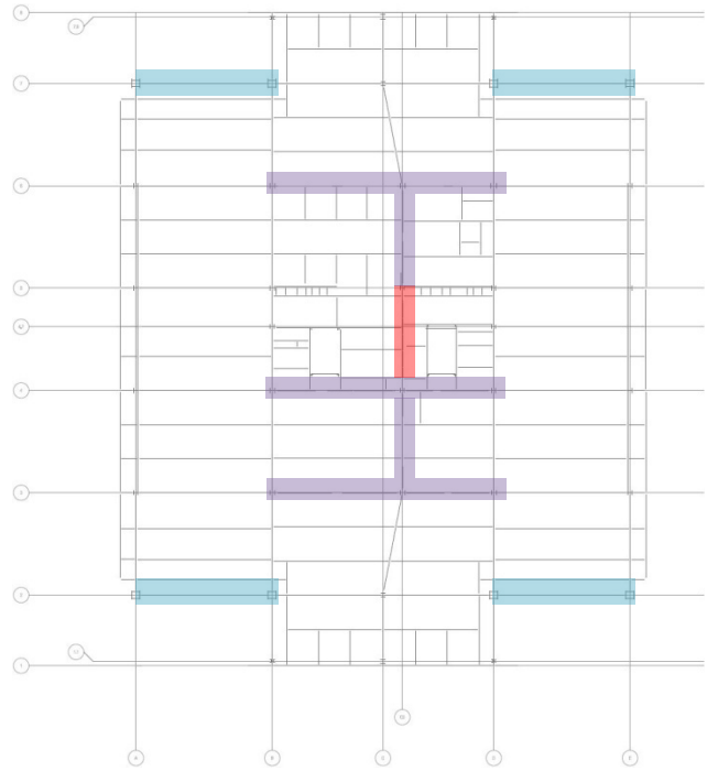
Figure 5: Typical Lateral System (Floors 1-27)
