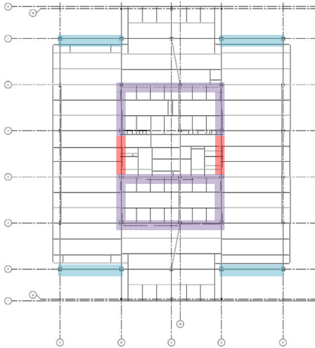
Figure 4: Typical Lateral System (Floors 29-50)
