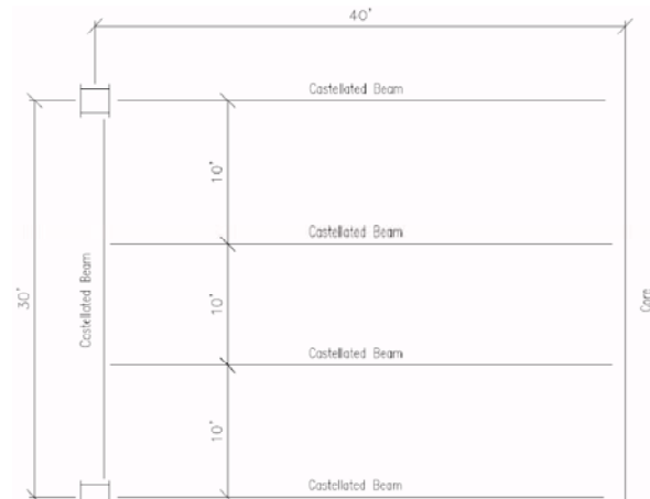
Figure 15: Castellated Beam w/ Typical Metal Decking Alternative
