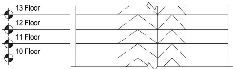
Figure 7: Typical Core E/W Core Bracing Elevation
