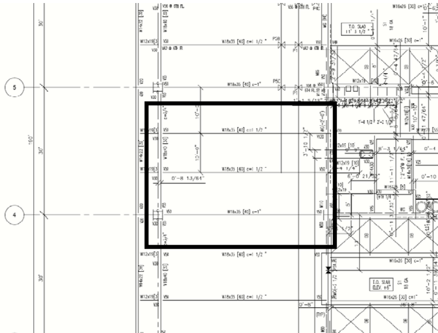
Figure 13 Typical 30'-0" x 40'-0" exterior bay
