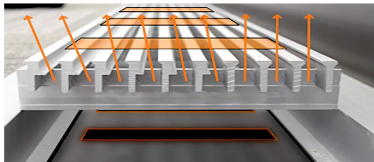
FIGURE 12: UFAD ILLUSTRATION
