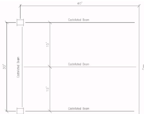
Figure 14: Castellated Beam w/ Long Span Metal Decking Alternative
