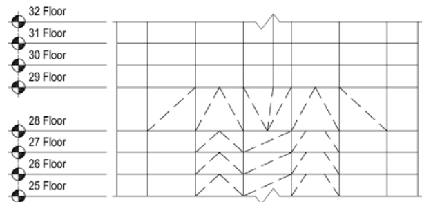
Figure 11: Typical N/S Outrigger Section (28th Floor)
